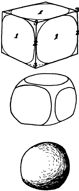
FIG. 155. — Successive diagrams to show the effect of decomposition and resulting disintegration upon joint blocks so as to produce spheroidal boulders by weathering.
